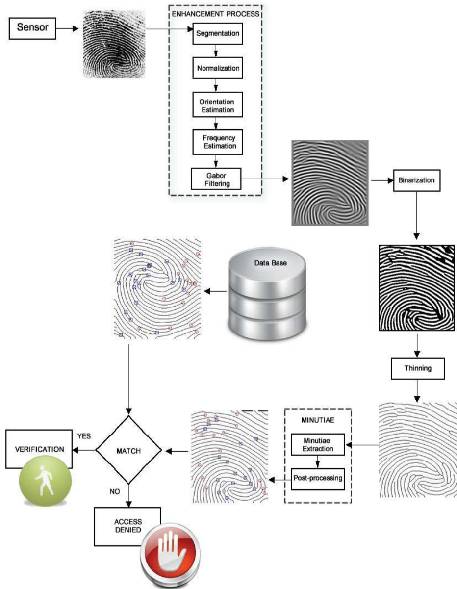
Fig. 1. Fingerprint authentication system
