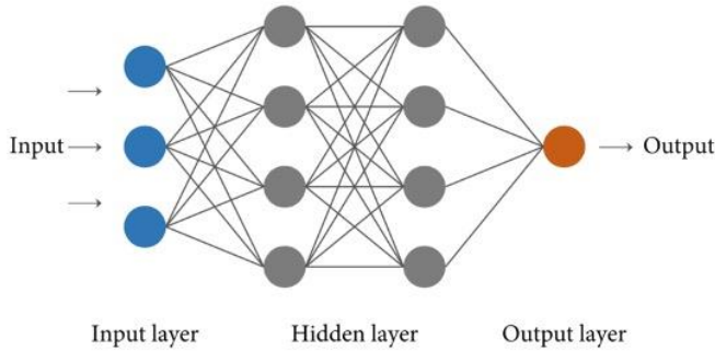
Fig. 3. ANN Architecture
