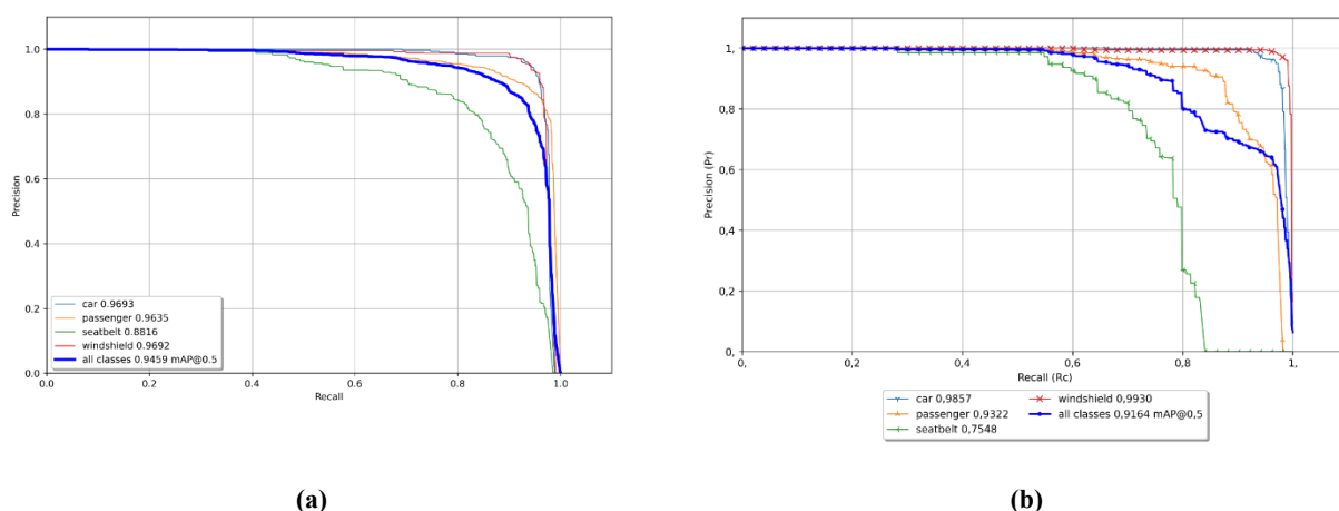
Fig. 7. Precision-recall curve of the best model daytime (a) and nighttime (b)
