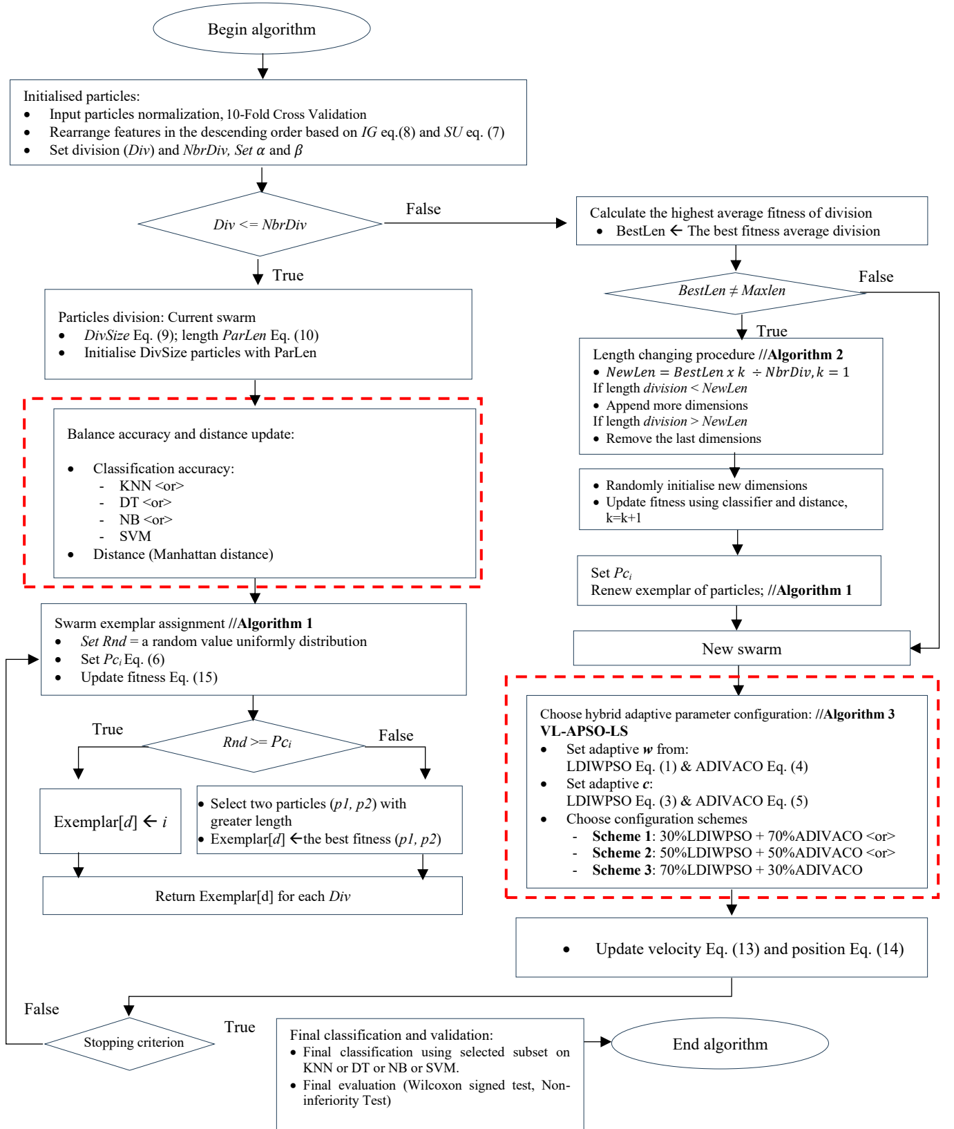
Fig. 4. Overall variable-length adaptive PSO algorithm
