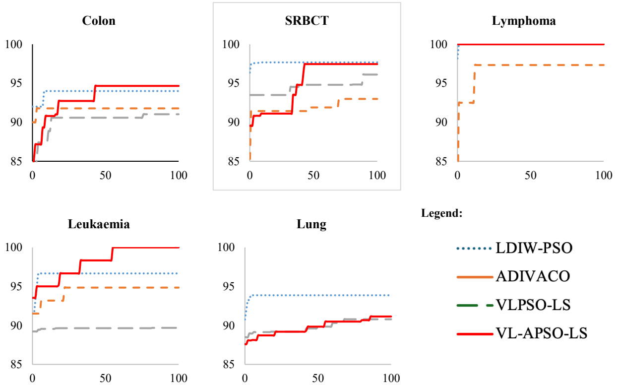
Fig. 7. Convergence behaviour analysis of VL-APSO-LS compared to state-of-the-art methods
