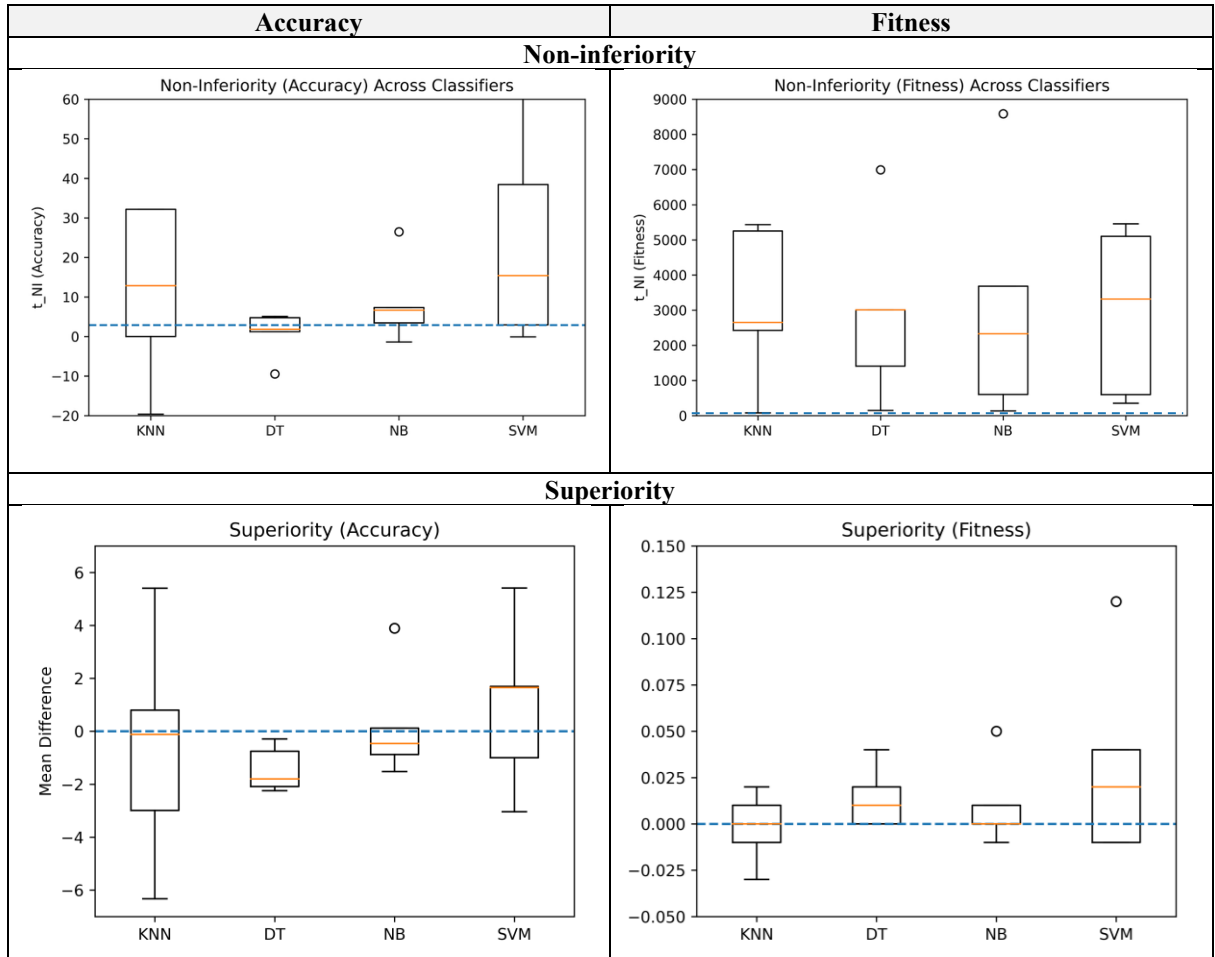
Fig. 6. Non-inferiority and superiority analysis of classification accuracy and fitness across classifiers
