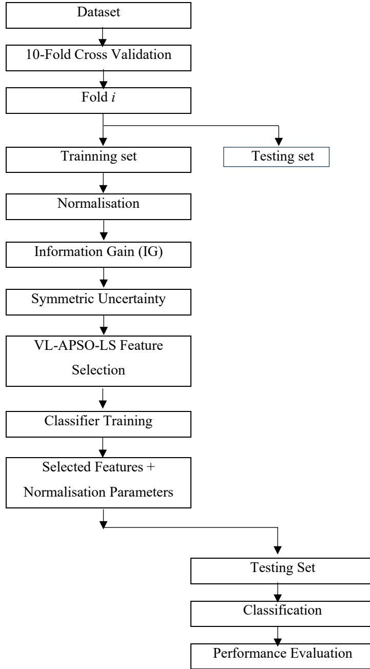
Fig. 3. Validation procedure used in each cross-validation iteration
