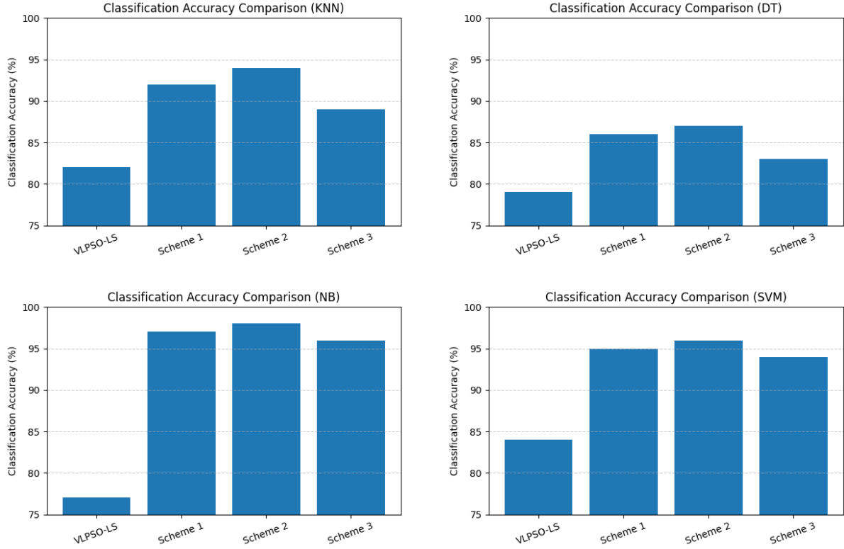
Fig. 5 The classification result comparison
