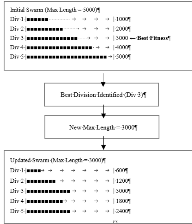
Fig. 1. Example of length changing in a swarm with five divisions
