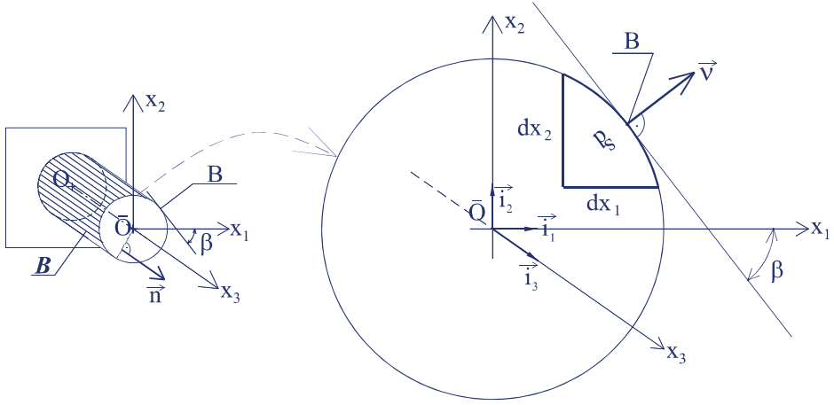
Fig. 5. Vector \vec{n} and geometrical relationships on the side of the rod
