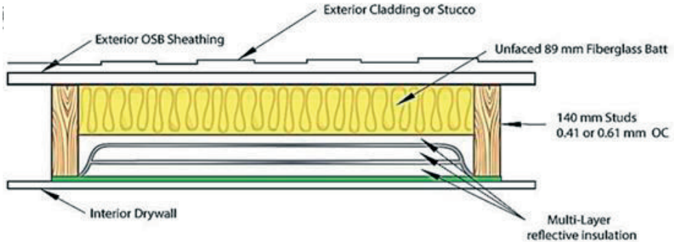
Fig. 3. Principle scheme of dynamic insulation, adapted from [11]
