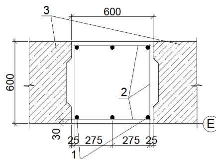
Fig. 10. Construction and reinforcement of the external wall of axis "E":
