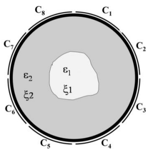
Fig. 1. Geometrical modelling of hopper flow in cross section. The set of estimated parameters \eta = \{\xi_1, \varepsilon_1, \xi_2, \varepsilon_2\} [12]
