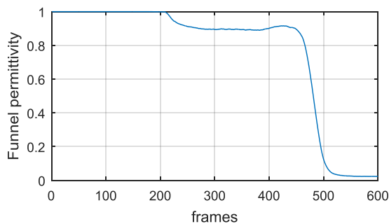
Fig. 4. Plot of the funnel permittivity \varepsilon_1 versus frames [12]
