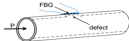
Fig. 22. Method for attaching the FBG to an exemplary pipe
