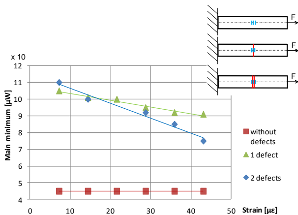
Fig. 14. Characteristics of the main minimum on transmission characteristics
