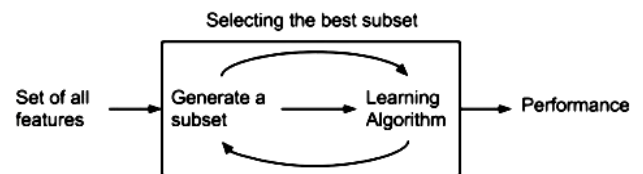
Fig. 4. Wrapper methods model [14]
