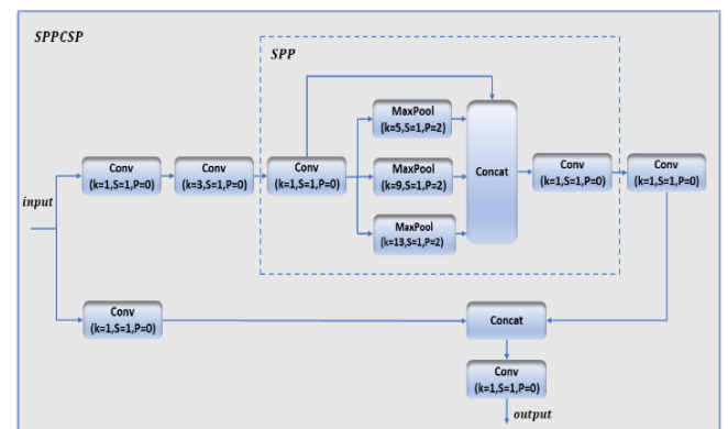
Fig. 5. SPPCSP modules Architecture
