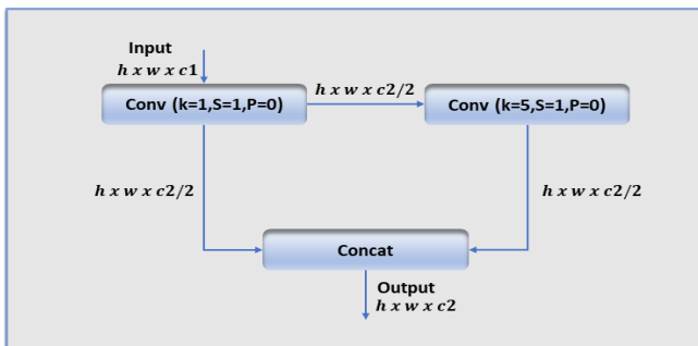
Fig. 7. The Ghostconv Module Structure
