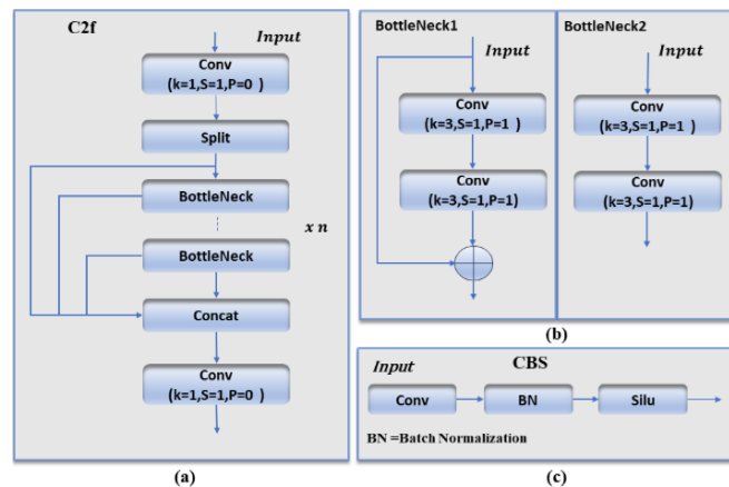
Fig. 1. The Structure of (a) C2f, (b) BottleNeck, (c) CBS
