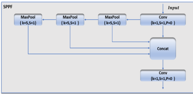
Fig. 2. Architecture of SPPF [22]
