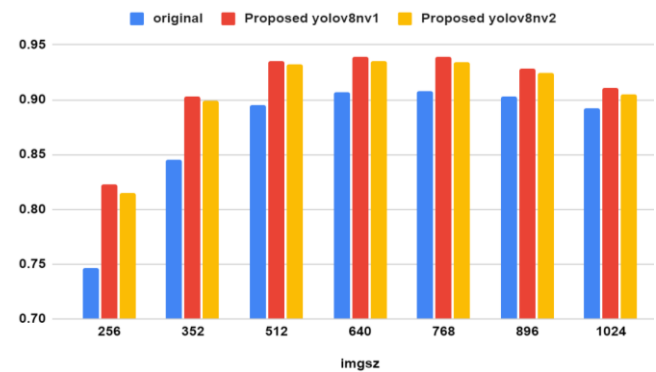
Fig. 10. Comparative analysis of original YOLOv8n, proposed YOLOv8n_v1 and proposed YOLOv8n_v2 of mAp50 for different size of images in the validation Results of MSFM dataset
