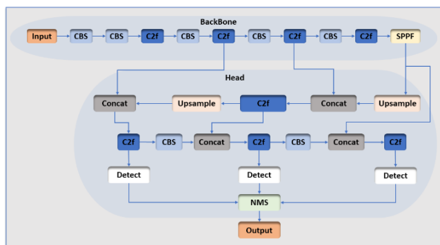
Fig. 3. YOLOv8n network architecture [13]
