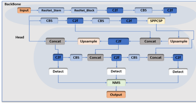
Fig. 6. The Architecture of the proposed YOLOv8n-v1
