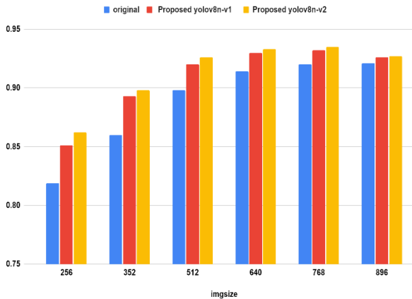
Fig. 9. Comparative analysis of original YOLOv8n, proposed YOLOv8n_v1 and proposed YOLOv8n_v2 of mAp50 for different size of images in the validation Results of MJFR Dataset
