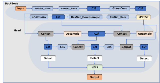
Fig. 8. Architecture of the proposed YOLOv8n-v2
