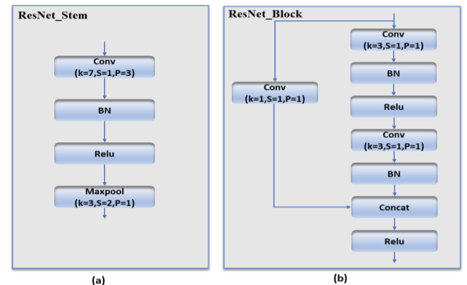
Fig. 4. The architecture of (a) ResNet_Stem module (b) The ResNet_Block module
