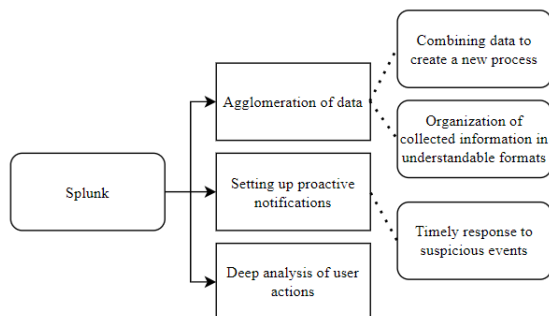
Fig. 4. Splunk functionality
