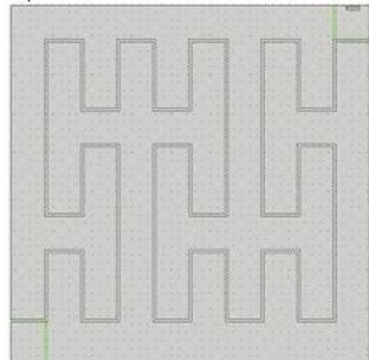
Fig. 5. Layout of Peano MIM 2
