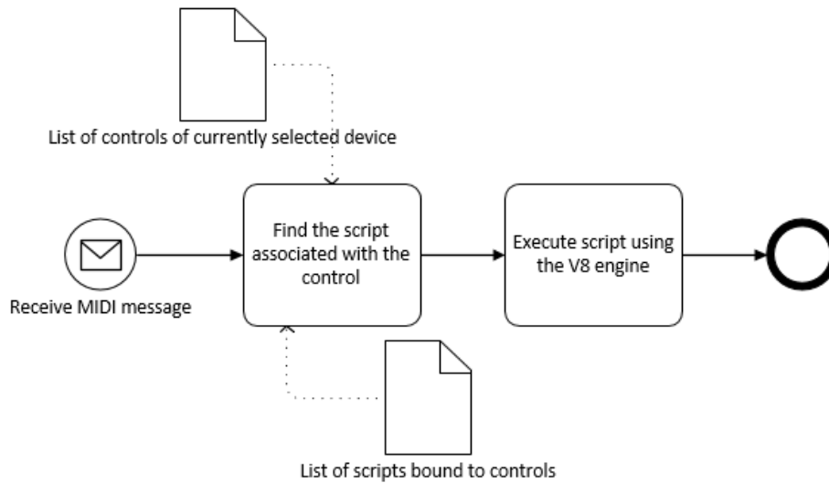
Fig. 3. Workflow of the DjToKey software
