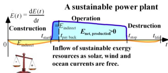
Figure 17. LCEA of a wind power plant. Source: Author's own work.
