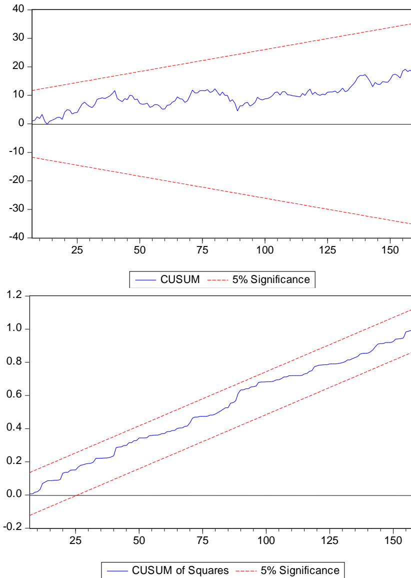
Figure 5. CUSUM and CUSUM Square Estimates (Author’s estimation)
