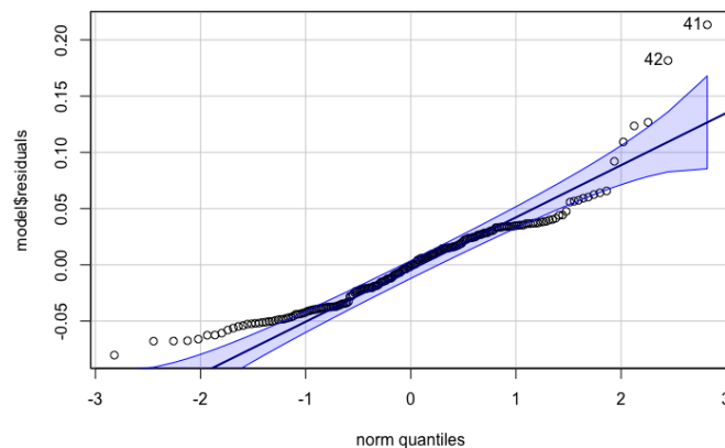
Figure 9. The testing the hypothesis of normal distribution of residuals for model with significant parameters
